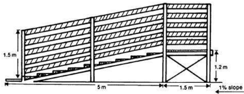
Gambar rajah menunjukkan contoh laluan tanjakan yang disyorkan. (Sumber: Economic Development, Jobs, Transport and Resources, Victoria State Government)
